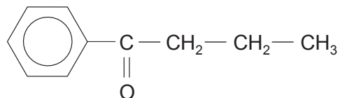
1-phenylbutanone
